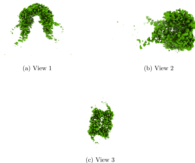
Figure 4: Isosurface at threshold=0.150000. Views generated by ChimeraX at a the following X, Y, Z angles: View 1 (0, -90, -90), View 2 (-90, 0, -90), View 3 (0, 0, 0).
