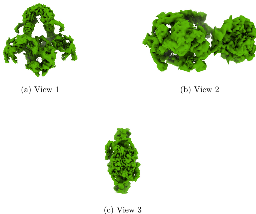
Figure 4: Isosurface at threshold=0.080000. Views generated by ChimeraX at a the following X, Y, Z angles: View 1 (0, -90, -90), View 2 (-90, 0, -90), View 3 (0, 0, 0).
