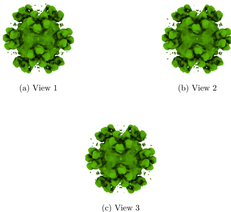
Figure 4: Isosurface at threshold=29.500000. Views generated by ChimeraX at a the following X, Y, Z angles: View 1 (0, -90, -90), View 2 (-90, 0, -90), View 3 (0, 0, 0).
