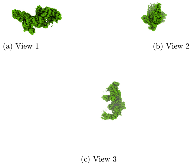
Figure 4: Isosurface at threshold=0.002500. Views generated by ChimeraX at a the following X, Y, Z angles: View 1 (0, -90, -90), View 2 (-90, 0, -90), View 3 (0, 0, 0).
