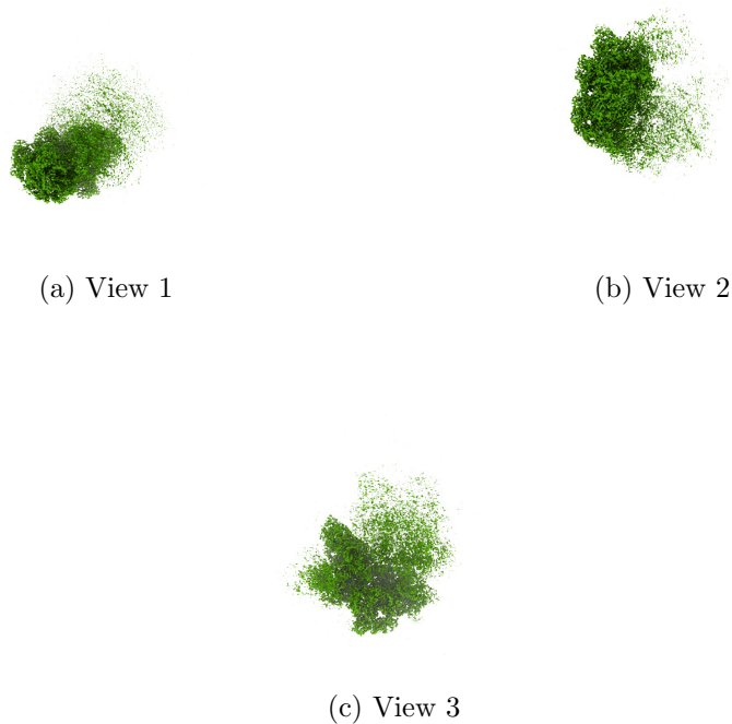
Figure 4: Isosurface at threshold=0.380000. Views generated by ChimeraX at a the following X, Y, Z angles: View 1 (0, -90, -90), View 2 (-90, 0, -90), View 3 (0, 0, 0).
