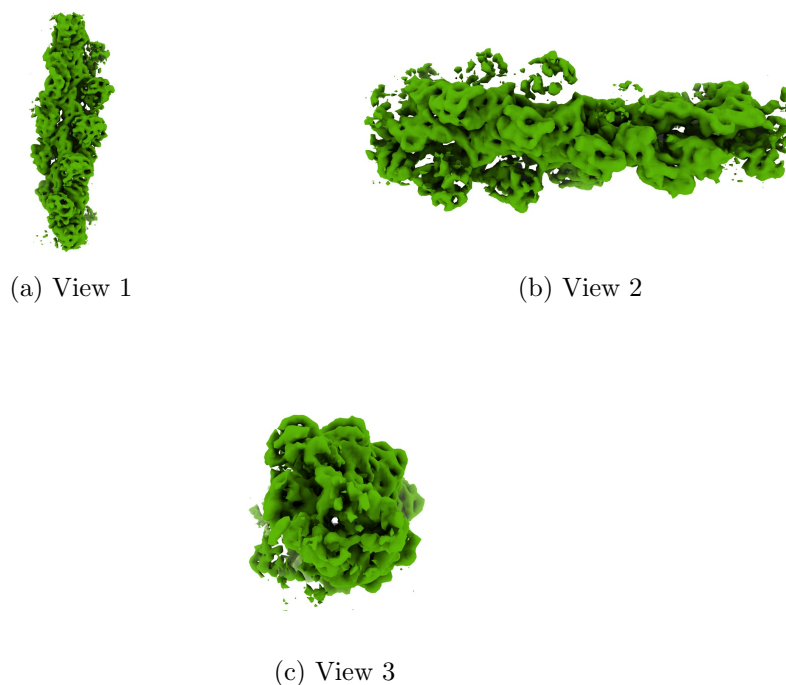
Figure 4: Isosurface at threshold=0.153000. Views generated by ChimeraX at a the following X, Y, Z angles: View 1 (0, -90, -90), View 2 (-90, 0, -90), View 3 (0, 0, 0).
