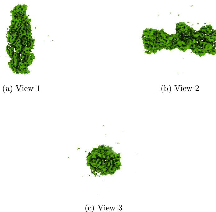
Figure 4: Isosurface at threshold=0.215000. Views generated by ChimeraX at a the following X, Y, Z angles: View 1 (0, -90, -90), View 2 (-90, 0, -90), View 3 (0, 0, 0).
