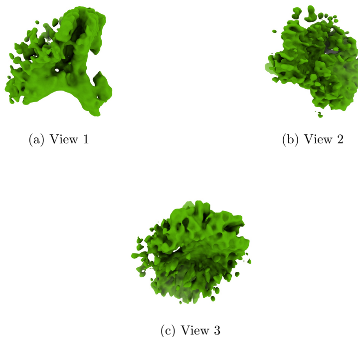
Figure 4: Isosurface at threshold=0.178000. Views generated by ChimeraX at a the following X, Y, Z angles: View 1 (0, -90, -90), View 2 (-90, 0, -90), View 3 (0, 0, 0).
