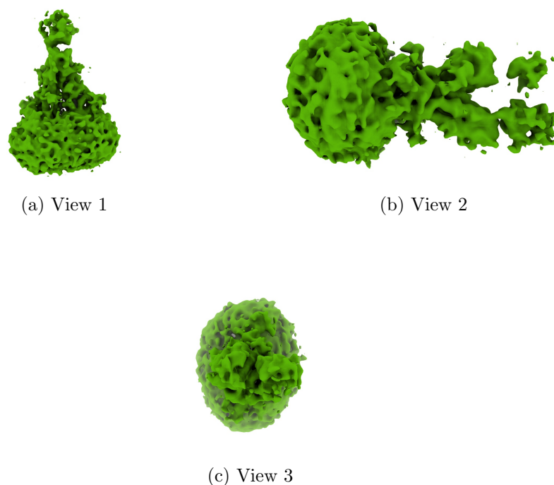
Figure 4: Isosurface at threshold=0.084500. Views generated by ChimeraX at a the following X, Y, Z angles: View 1 (0, -90, -90), View 2 (-90, 0, -90), View 3 (0, 0, 0).
