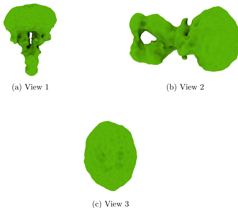
Figure 4: Isosurface at threshold=0.062700. Views generated by ChimeraX at the following X, Y, Z angles: View 1 (0, -90, -90), View 2 (-90, 0, -90), View 3 (0, 0, 0).
