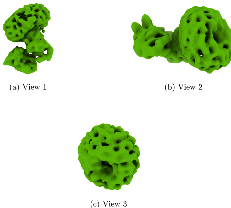
Figure 4: Isosurface at threshold=0.004850. Views generated by ChimeraX at a the following X, Y, Z angles: View 1 (0, -90, -90), View 2 (-90, 0, -90), View 3 (0, 0, 0).
