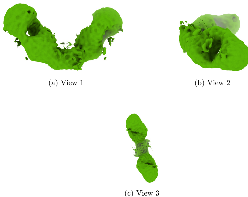
Figure 4: Isosurface at threshold=0.120000. Views generated by ChimeraX at a the following X, Y, Z angles: View 1 (0, -90, -90), View 2 (-90, 0, -90), View 3 (0, 0, 0).
