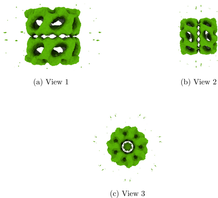
Figure 4: Isosurface at threshold=0.005450. Views generated by ChimeraX at a the following X, Y, Z angles: View 1 (0, -90, -90), View 2 (-90, 0, -90), View 3 (0, 0, 0).
