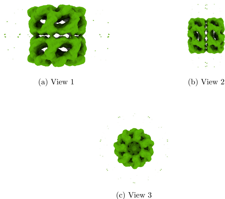
Figure 4: Isosurface at threshold=0.004330. Views generated by ChimeraX at a the following X, Y, Z angles: View 1 (0, -90, -90), View 2 (-90, 0, -90), View 3 (0, 0, 0).
