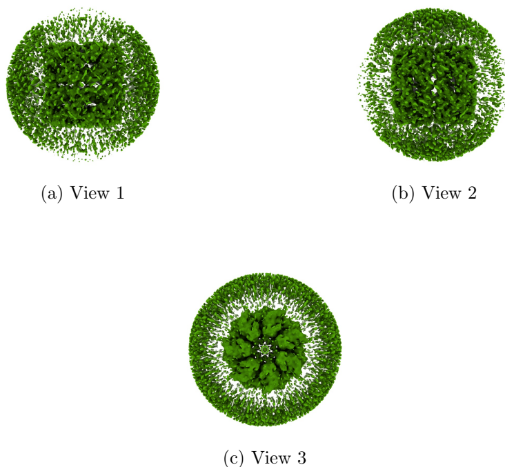
Figure 4: Isosurface at threshold=1.880000. Views generated by ChimeraX at a the following X, Y, Z angles: View 1 (0, -90, -90), View 2 (-90, 0, -90), View 3 (0, 0, 0).
