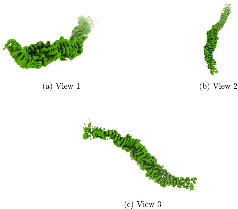
Figure 4: Isosurface at threshold=0.004930. Views generated by ChimeraX at a the following X, Y, Z angles: View 1 (0, -90, -90), View 2 (-90, 0, -90), View 3 (0, 0, 0).
