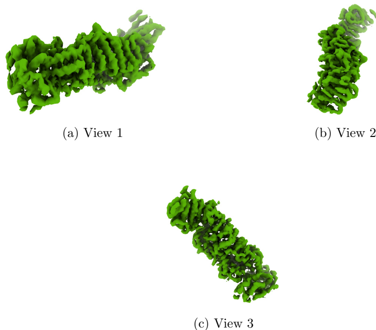
Figure 4: Isosurface at threshold=0.006930. Views generated by ChimeraX at a the following X, Y, Z angles: View 1 (0, -90, -90), View 2 (-90, 0, -90), View 3 (0, 0, 0).
