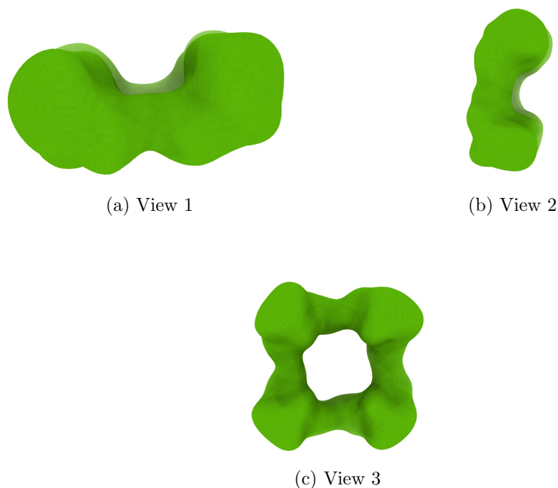
Figure 4: Isosurface at threshold=0.157000. Views generated by ChimeraX at a the following X, Y, Z angles: View 1 (0, -90, -90), View 2 (-90, 0, -90), View 3 (0, 0, 0).
