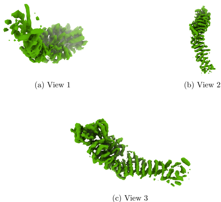
Figure 4: Isosurface at threshold=0.007180. Views generated by ChimeraX at a the following X, Y, Z angles: View 1 (0, -90, -90), View 2 (-90, 0, -90), View 3 (0, 0, 0).
