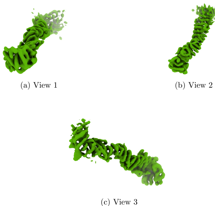
Figure 4: Isosurface at threshold=0.005250. Views generated by ChimeraX at a the following X, Y, Z angles: View 1 (0, -90, -90), View 2 (-90, 0, -90), View 3 (0, 0, 0).
