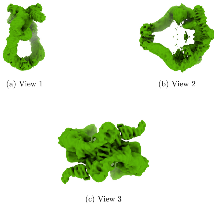
Figure 4: Isosurface at threshold=0.002160. Views generated by ChimeraX at a the following X, Y, Z angles: View 1 (0, -90, -90), View 2 (-90, 0, -90), View 3 (0, 0, 0).
