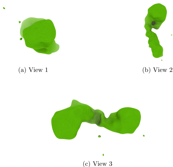
Figure 4: Isosurface at threshold=0.015740. Views generated by ChimeraX at a the following X, Y, Z angles: View 1 (0, -90, -90), View 2 (-90, 0, -90), View 3 (0, 0, 0).
