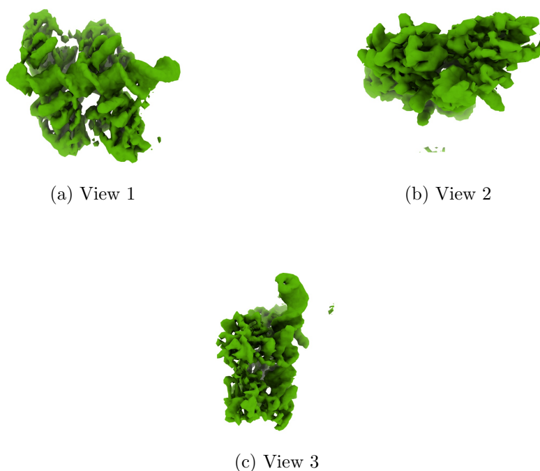
Figure 4: Isosurface at threshold=0.352000. Views generated by ChimeraX at a the following X, Y, Z angles: View 1 (0, -90, -90), View 2 (-90, 0, -90), View 3 (0, 0, 0).
