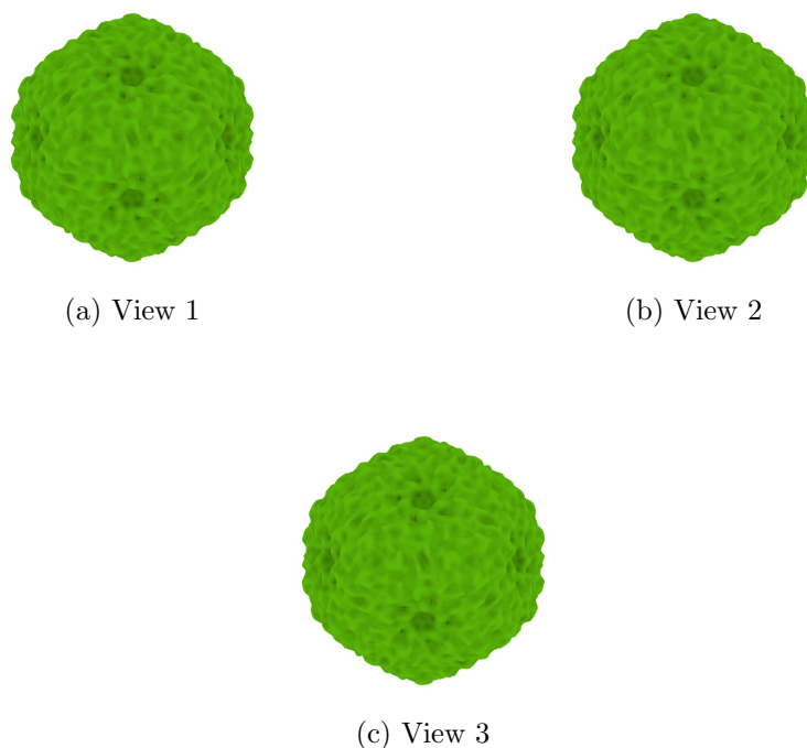
Figure 4: Isosurface at threshold=1.620000. Views generated by ChimeraX at a the following X, Y, Z angles: View 1 (0, -90, -90), View 2 (-90, 0, -90), View 3 (0, 0, 0).
