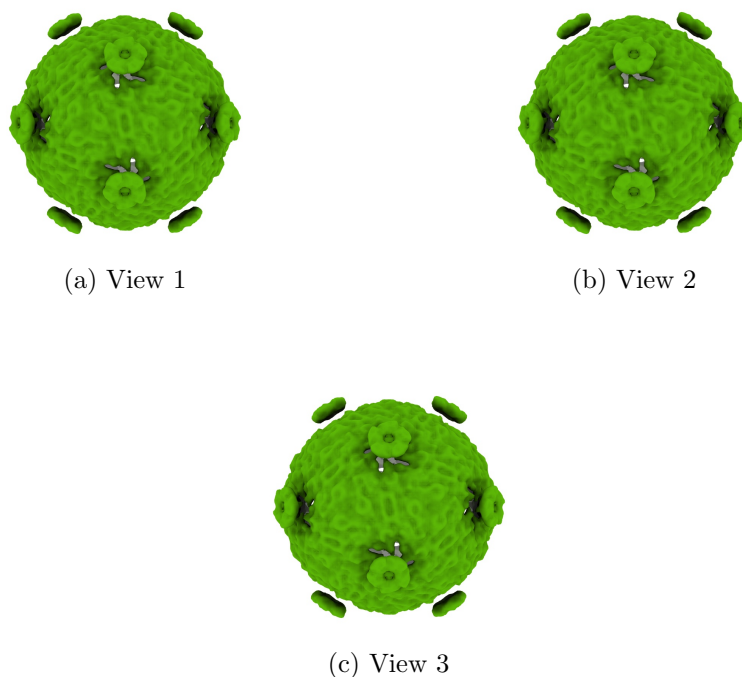
Figure 4: Isosurface at threshold=2.070000. Views generated by ChimeraX at a the following X, Y, Z angles: View 1 (0, -90, -90), View 2 (-90, 0, -90), View 3 (0, 0, 0).
