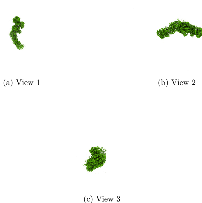
Figure 4: Isosurface at threshold=0.040000. Views generated by ChimeraX at a the following X, Y, Z angles: View 1 (0, -90, -90), View 2 (-90, 0, -90), View 3 (0, 0, 0).
