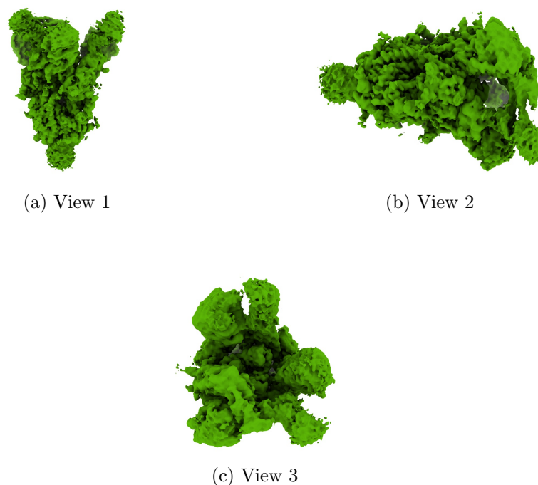
Figure 4: Isosurface at threshold=0.059800. Views generated by ChimeraX at a the following X, Y, Z angles: View 1 (0, -90, -90), View 2 (-90, 0, -90), View 3 (0, 0, 0).
