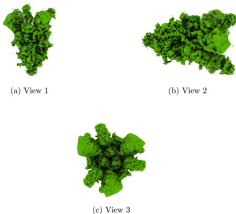
Figure 4: Isosurface at threshold=0.060500. Views generated by ChimeraX at a the following X, Y, Z angles: View 1 (0, -90, -90), View 2 (-90, 0, -90), View 3 (0, 0, 0).
