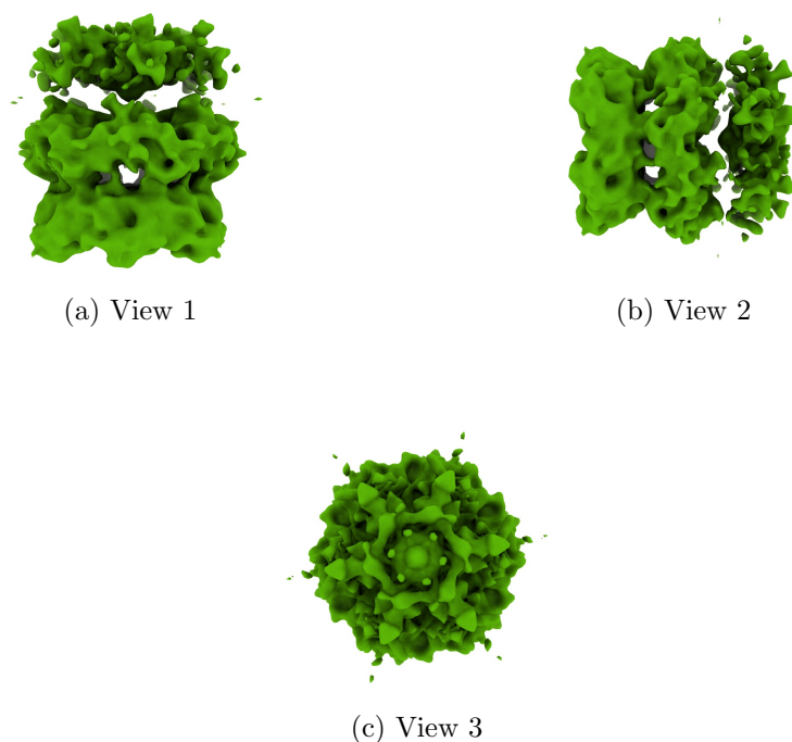
Figure 4: Isosurface at threshold=2.600000. Views generated by ChimeraX at a the following X, Y, Z angles: View 1 (0, -90, -90), View 2 (-90, 0, -90), View 3 (0, 0, 0).
