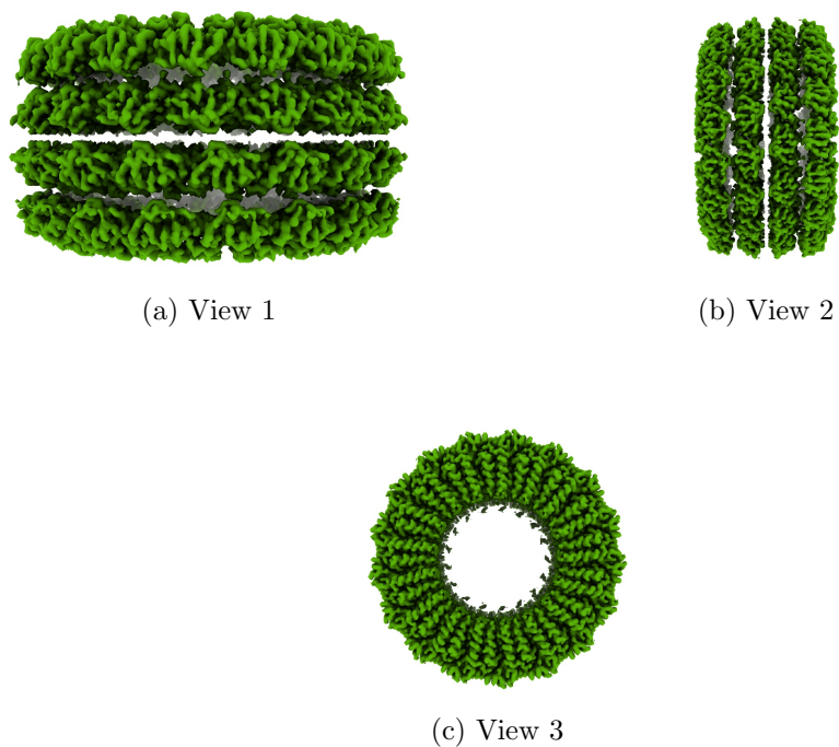
Figure 4: Isosurface at threshold=0.142000. Views generated by ChimeraX at a the following X, Y, Z angles: View 1 (0, -90, -90), View 2 (-90, 0, -90), View 3 (0, 0, 0).
