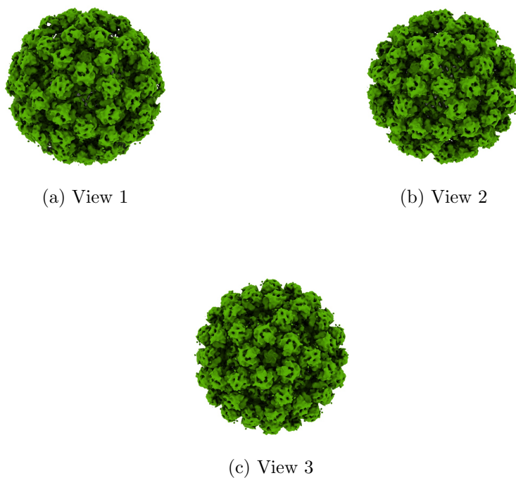
Figure 4: Isosurface at threshold=2.870000. Views generated by ChimeraX at a the following X, Y, Z angles: View 1 (0, -90, -90), View 2 (-90, 0, -90), View 3 (0, 0, 0).
