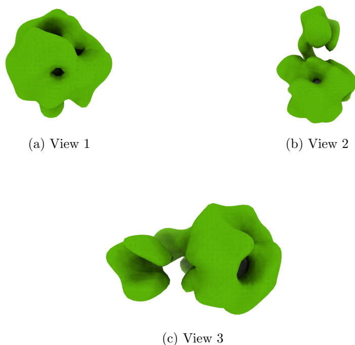
Figure 4: Isosurface at threshold=3.670000. Views generated by ChimeraX at a the following X, Y, Z angles: View 1 (0, -90, -90), View 2 (-90, 0, -90), View 3 (0, 0, 0).
