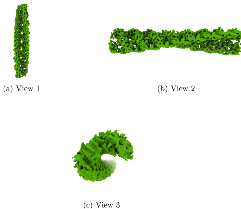
Figure 4: Isosurface at threshold=0.083800. Views generated by ChimeraX at a the following X, Y, Z angles: View 1 (0, -90, -90), View 2 (-90, 0, -90), View 3 (0, 0, 0).
