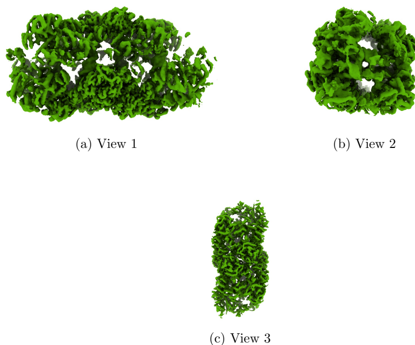
Figure 4: Isosurface at threshold=3.830000. Views generated by ChimeraX at a the following X, Y, Z angles: View 1 (0, -90, -90), View 2 (-90, 0, -90), View 3 (0, 0, 0).
