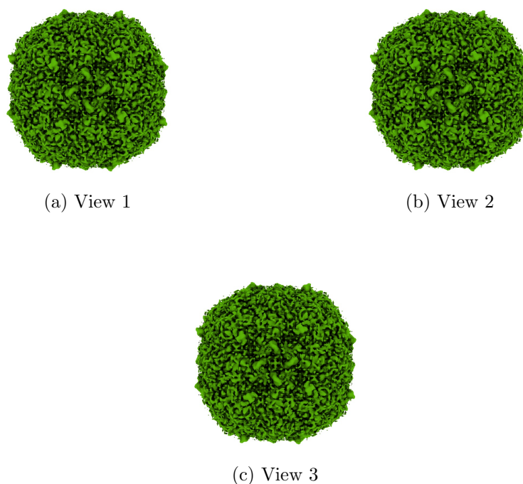
Figure 4: Isosurface at threshold=0.034900. Views generated by ChimeraX at a the following X, Y, Z angles: View 1 (0, -90, -90), View 2 (-90, 0, -90), View 3 (0, 0, 0).
