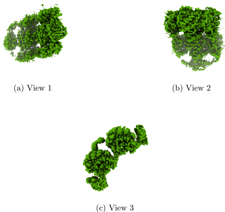
Figure 4: Isosurface at threshold=0.105000. Views generated by ChimeraX at a the following X, Y, Z angles: View 1 (0, -90, -90), View 2 (-90, 0, -90), View 3 (0, 0, 0).
