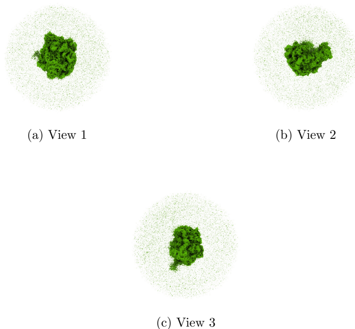
Figure 4: Isosurface at threshold=0.053600. Views generated by ChimeraX at a the following X, Y, Z angles: View 1 (0, -90, -90), View 2 (-90, 0, -90), View 3 (0, 0, 0).
