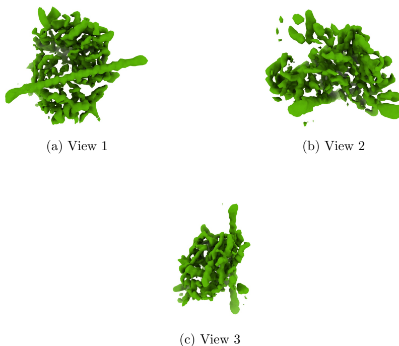
Figure 4: Isosurface at threshold=0.107000. Views generated by ChimeraX at a the following X, Y, Z angles: View 1 (0, -90, -90), View 2 (-90, 0, -90), View 3 (0, 0, 0).
