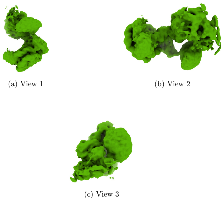
Figure 4: Isosurface at threshold=0.075800. Views generated by ChimeraX at a the following X, Y, Z angles: View 1 (0, -90, -90), View 2 (-90, 0, -90), View 3 (0, 0, 0).
