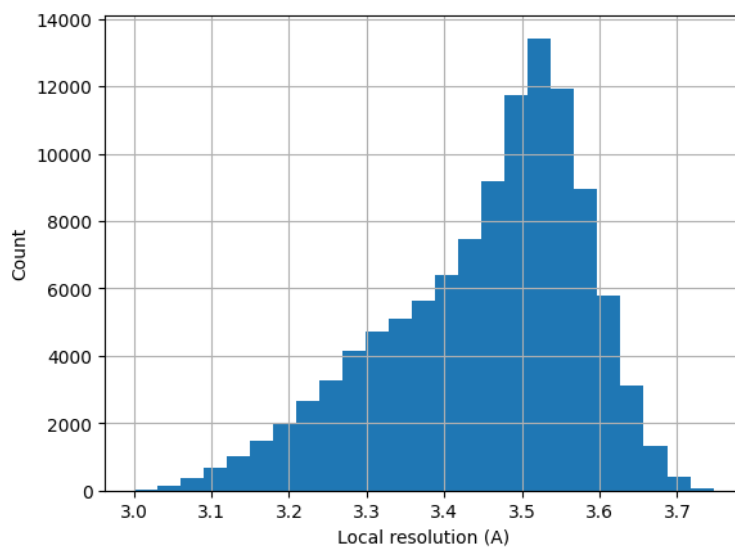
Figure 24: Histogram of the local resolution according to Resmap.
