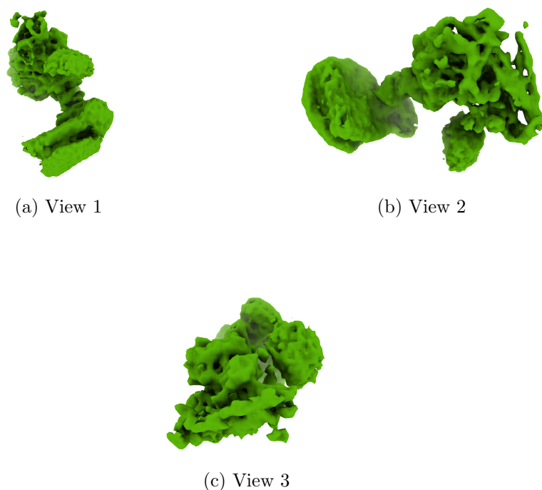
Figure 4: Isosurface at threshold=0.087600. Views generated by ChimeraX at a the following X, Y, Z angles: View 1 (0, -90, -90), View 2 (-90, 0, -90), View 3 (0, 0, 0).
