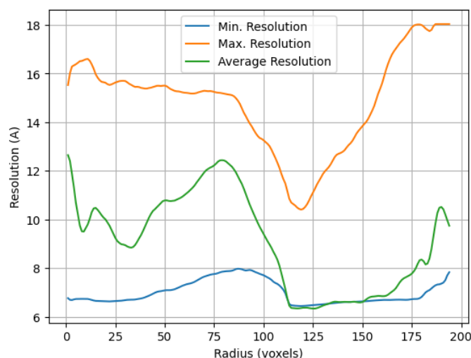
Figure 28: Radial averages (in space) of the minimum, maximum and average resolution at each voxel.
