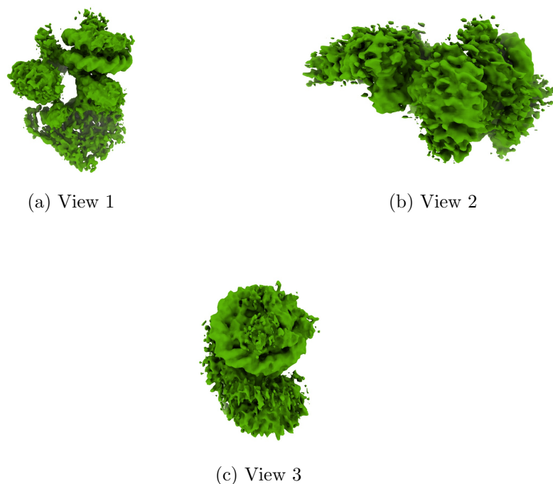
Figure 4: Isosurface at threshold=0.098100. Views generated by ChimeraX at a the following X, Y, Z angles: View 1 (0, -90, -90), View 2 (-90, 0, -90), View 3 (0, 0, 0).
