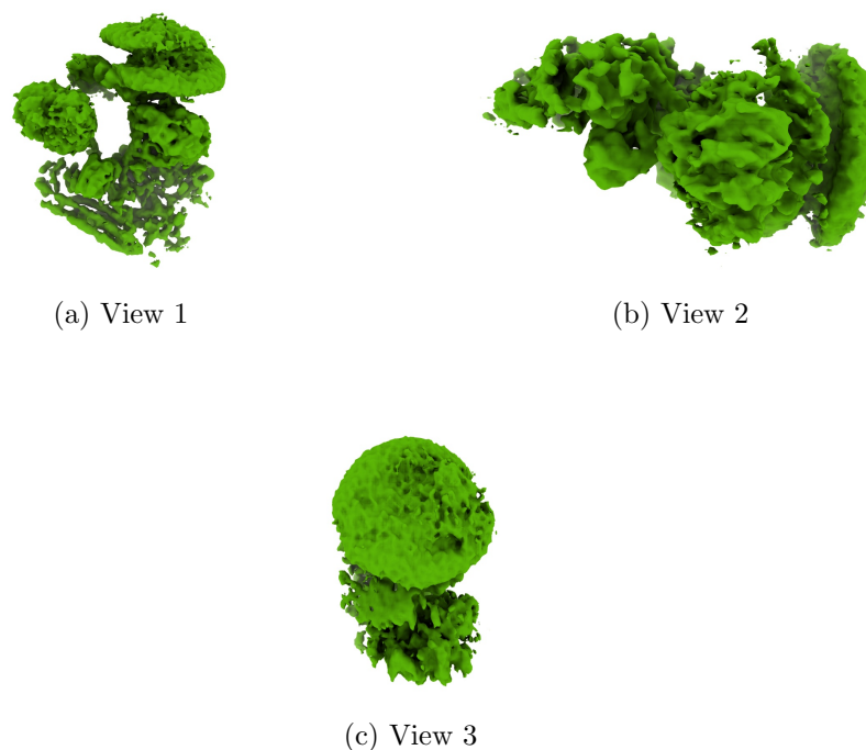
Figure 4: Isosurface at threshold=0.133000. Views generated by ChimeraX at a the following X, Y, Z angles: View 1 (0, -90, -90), View 2 (-90, 0, -90), View 3 (0, 0, 0).
