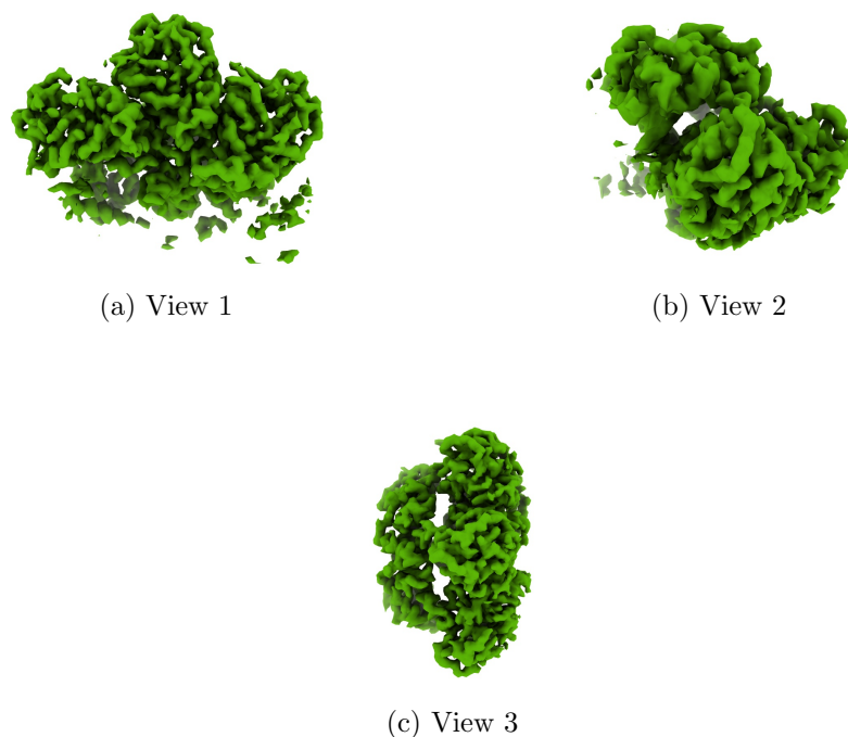
Figure 4: Isosurface at threshold=0.040600. Views generated by ChimeraX at a the following X, Y, Z angles: View 1 (0, -90, -90), View 2 (-90, 0, -90), View 3 (0, 0, 0).
