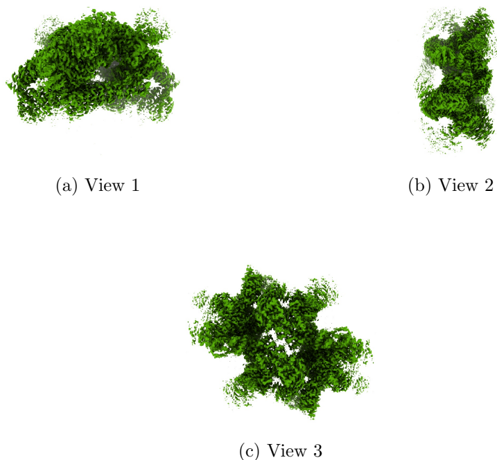
Figure 4: Isosurface at threshold=0.084200. Views generated by ChimeraX at a the following X, Y, Z angles: View 1 (0, -90, -90), View 2 (-90, 0, -90), View 3 (0, 0, 0).
