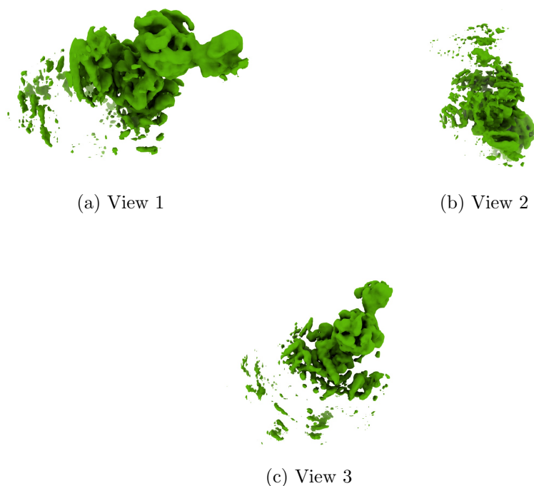
Figure 4: Isosurface at threshold=0.041300. Views generated by ChimeraX at a the following X, Y, Z angles: View 1 (0, -90, -90), View 2 (-90, 0, -90), View 3 (0, 0, 0).
