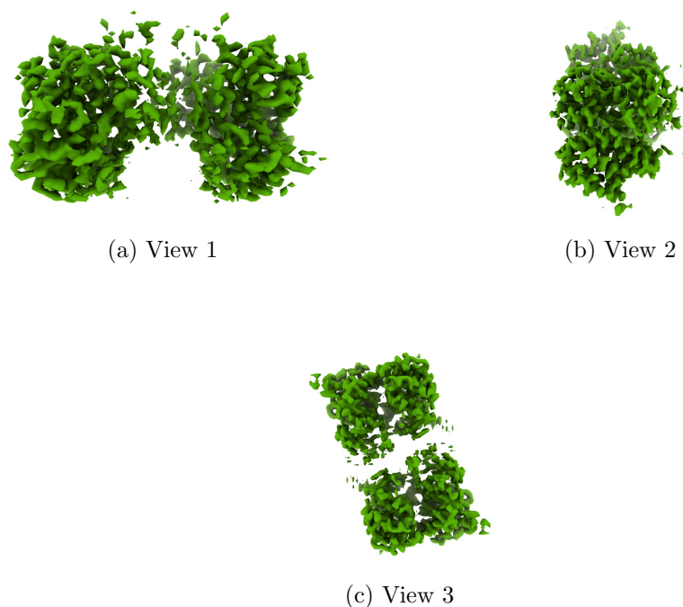
Figure 4: Isosurface at threshold=0.027700. Views generated by ChimeraX at a the following X, Y, Z angles: View 1 (0, -90, -90), View 2 (-90, 0, -90), View 3 (0, 0, 0).
