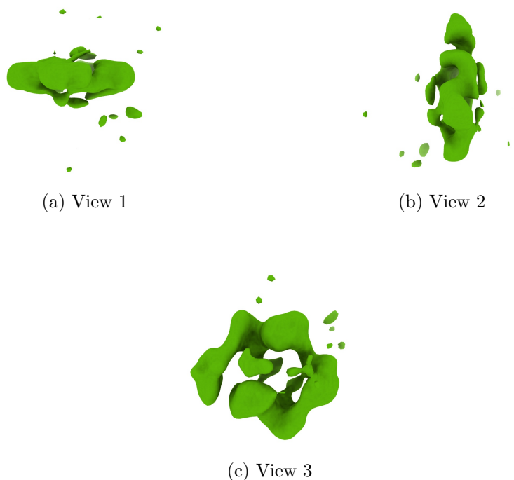
Figure 4: Isosurface at threshold=1.700000. Views generated by ChimeraX at a the following X, Y, Z angles: View 1 (0, -90, -90), View 2 (-90, 0, -90), View 3 (0, 0, 0).
