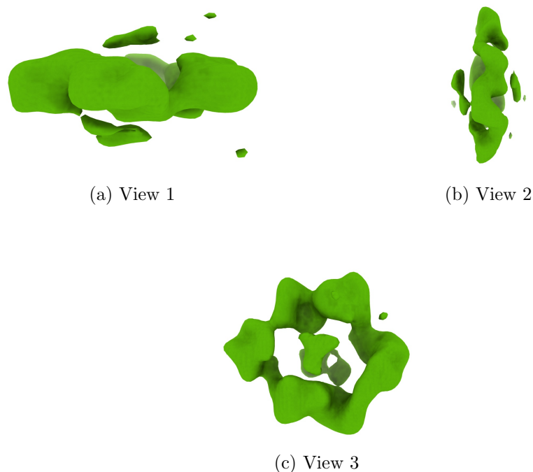
Figure 4: Isosurface at threshold=1.950000. Views generated by ChimeraX at a the following X, Y, Z angles: View 1 (0, -90, -90), View 2 (-90, 0, -90), View 3 (0, 0, 0).
