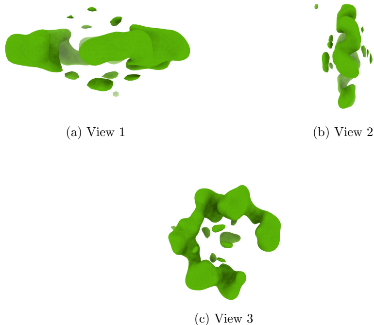
Figure 4: Isosurface at threshold=2.260000. Views generated by ChimeraX at a the following X, Y, Z angles: View 1 (0, -90, -90), View 2 (-90, 0, -90), View 3 (0, 0, 0).
