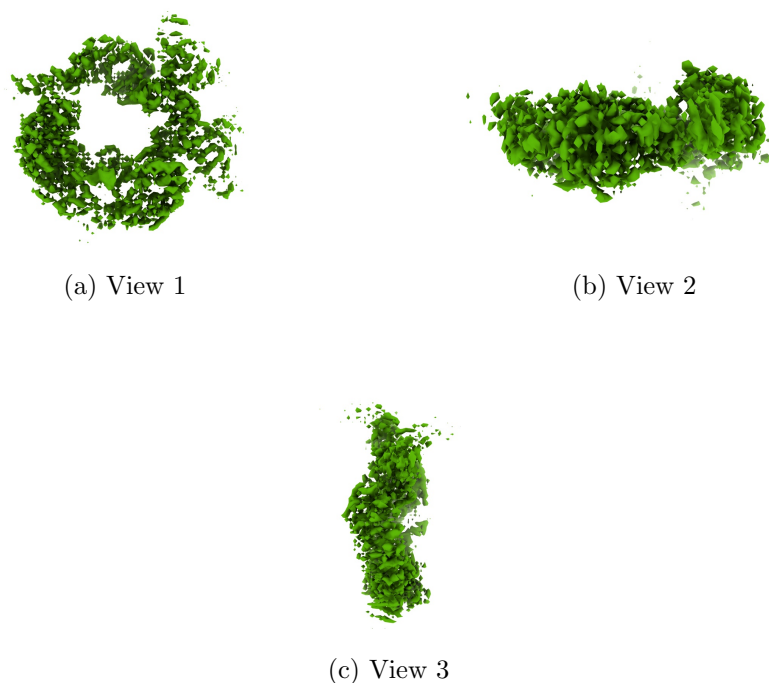
Figure 4: Isosurface at threshold=0.079600. Views generated by ChimeraX at a the following X, Y, Z angles: View 1 (0, -90, -90), View 2 (-90, 0, -90), View 3 (0, 0, 0).
